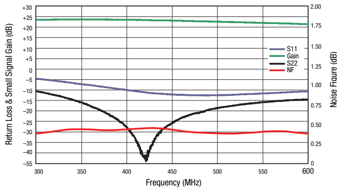
Figure 17. Evaluation Board NF, Gain, and Return Losses for 380 to 530 MHz Tuning
