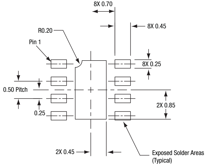
Figure 25. SKY67150-396LF PCB Layout Footprint (Top View)
